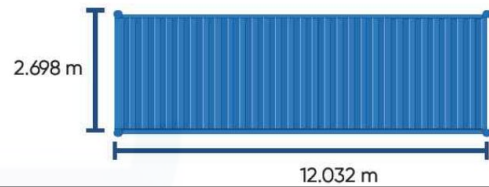
CONTAINER 40 FT STANDARD HIGH CUBE:
