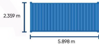
CONTAINER 20 FT STANDARD:
